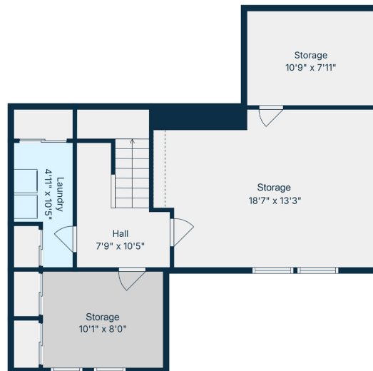
Basement
