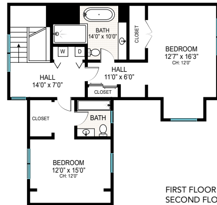
SECOND FLOOR CEILING HEIGHT: 11'9"
