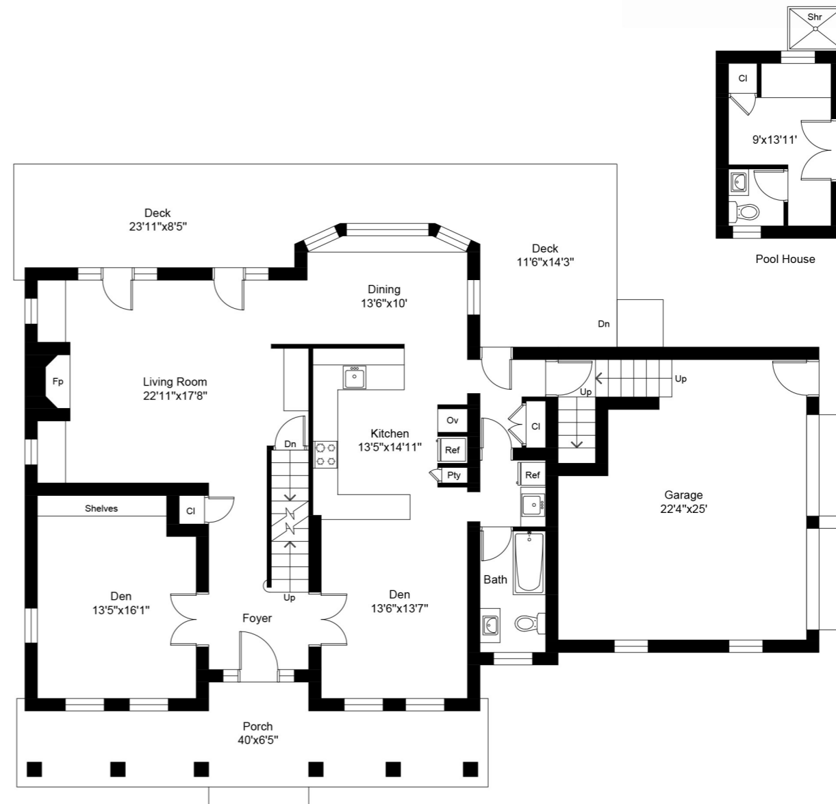
FIRST FLOOR
